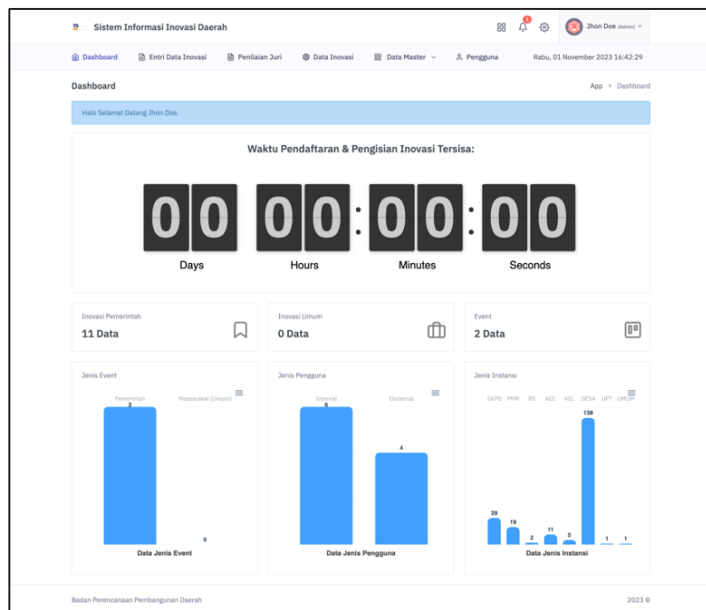
Gambar 3. 3 Halaman Menu/Dashboard
